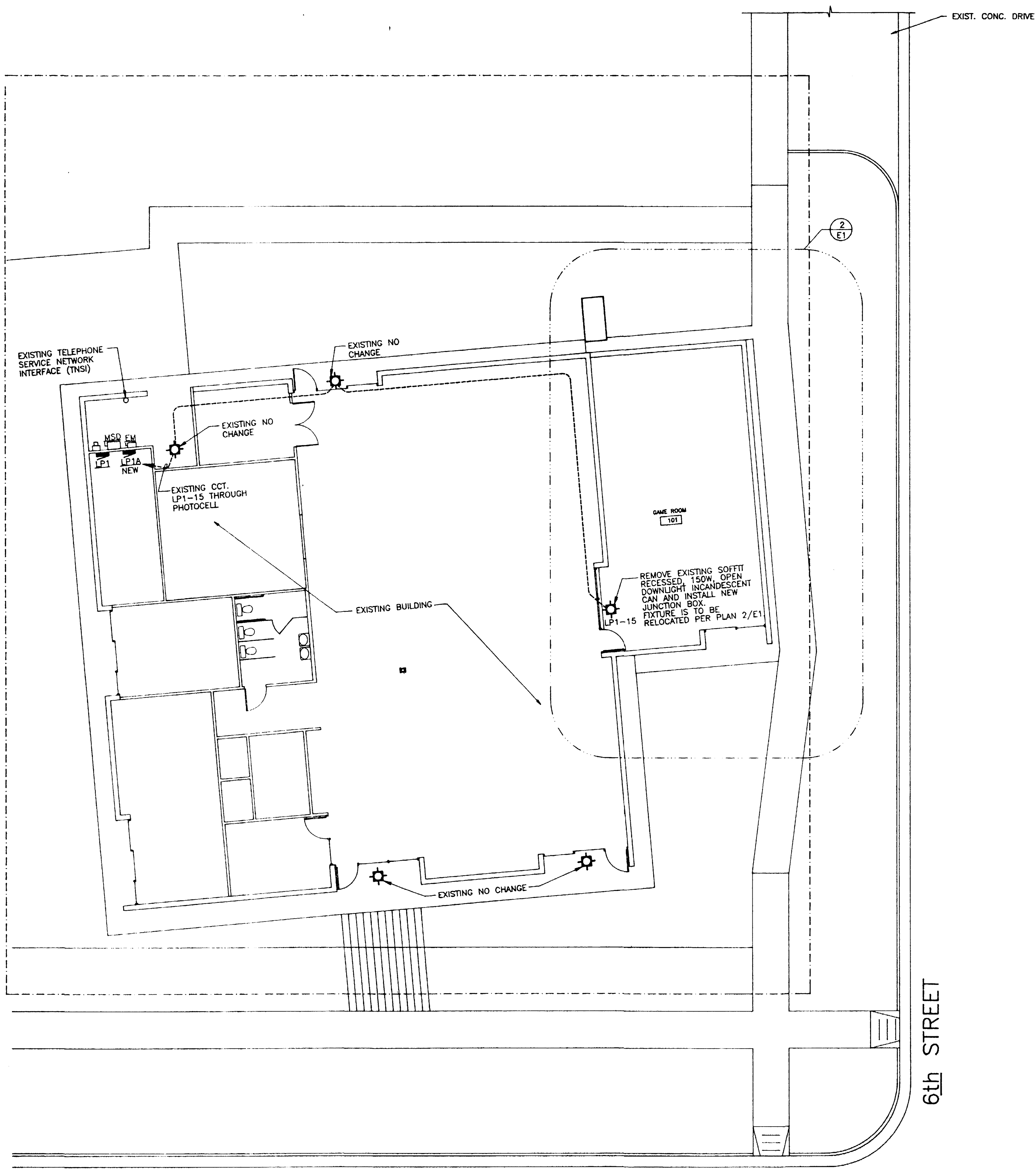
1 ELECTRICAL FLOOR PLAN 1/8"=1'-0"
