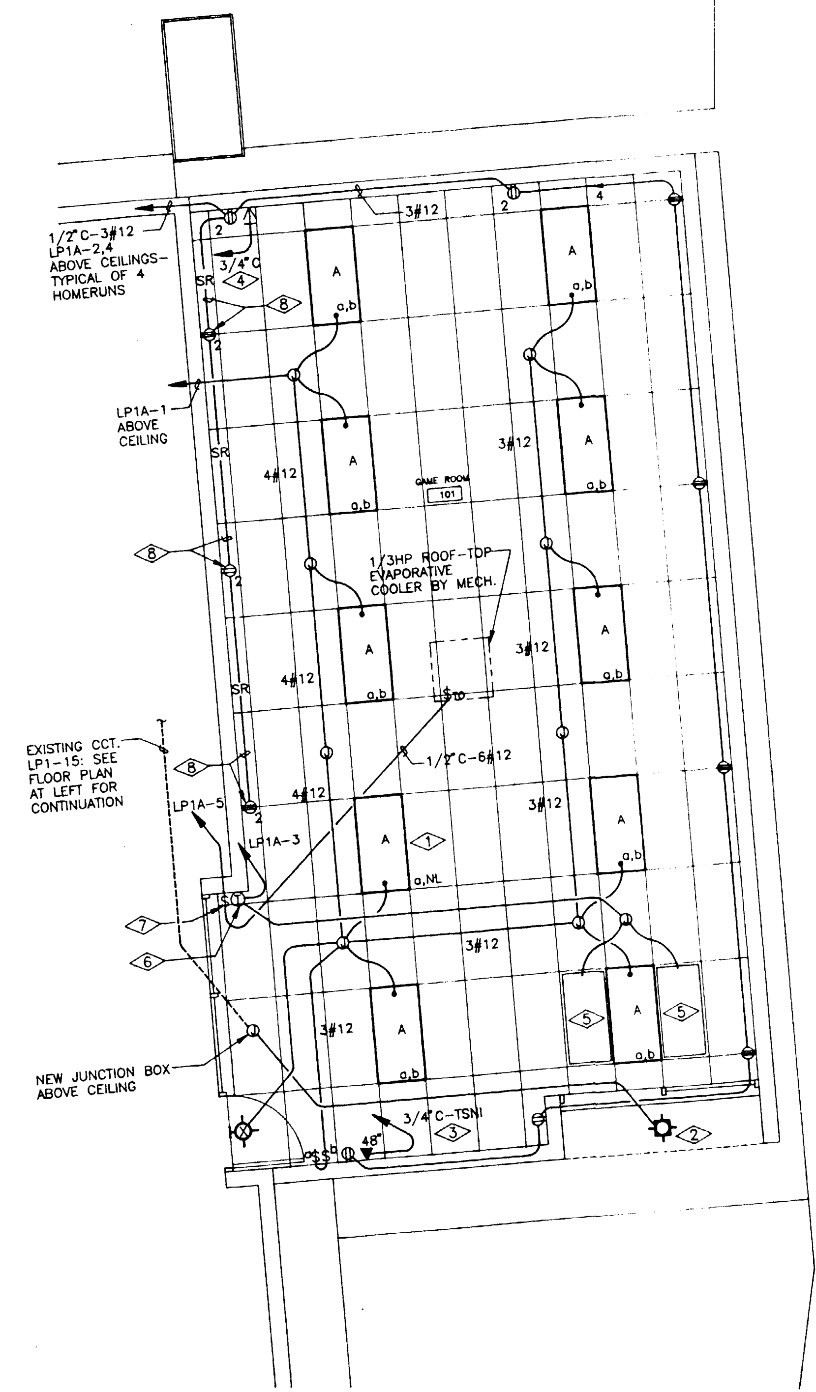
2 GAME ROOM ELECTRICAL PLAN 1/4"=1'-0"
