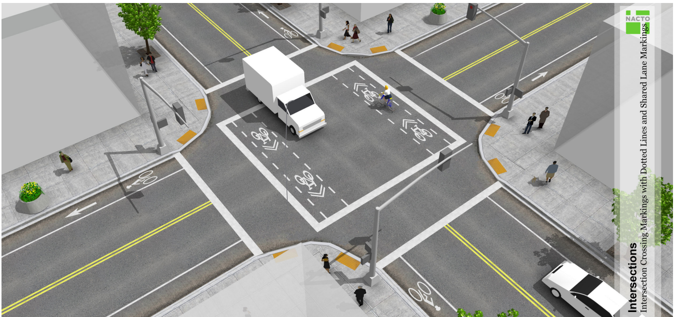
FIGURE 21: DEDICATED INTERSECTION
