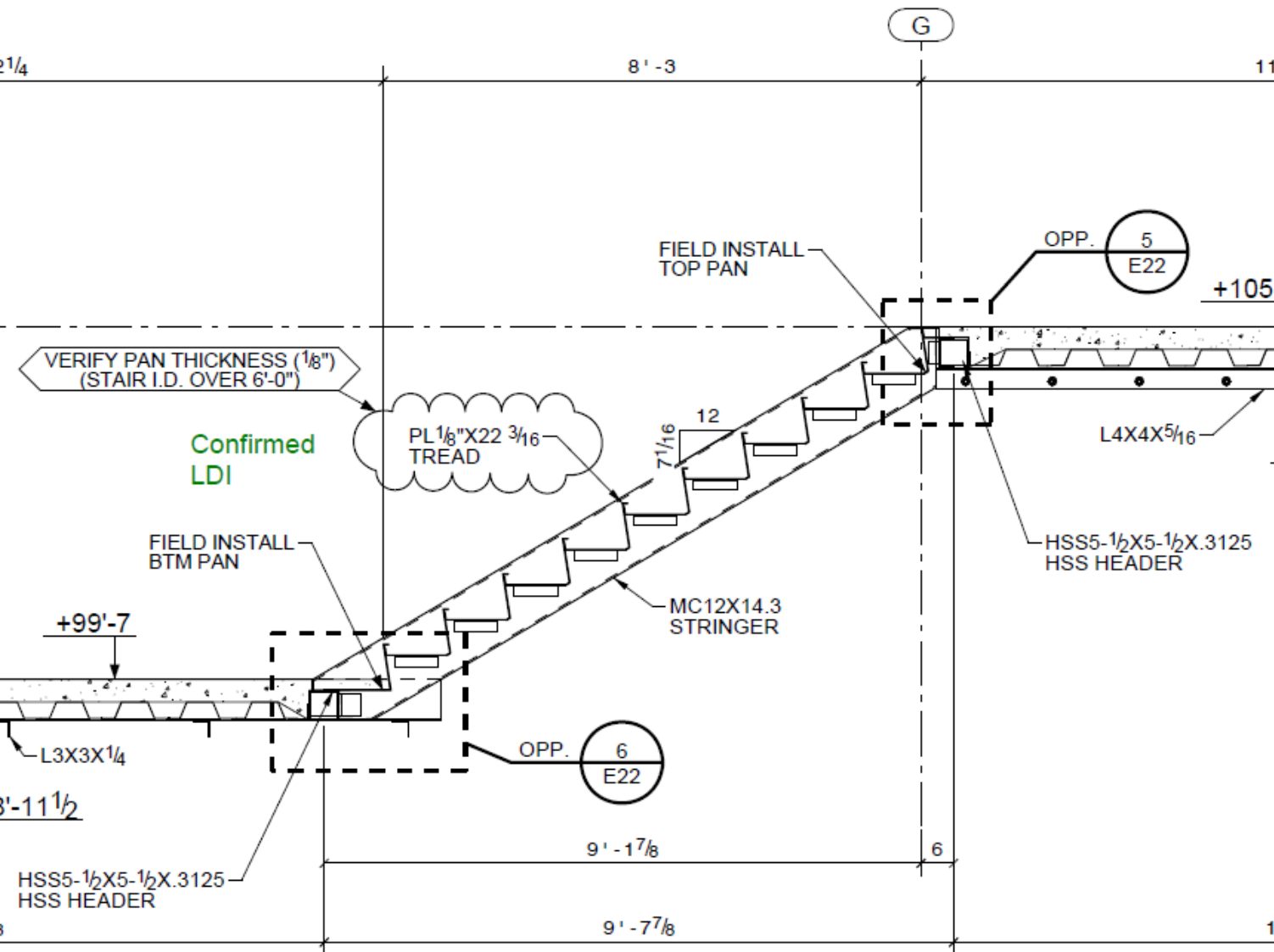
B EAST STAIR ELEVATION VIEW (SOUTH WALL)
