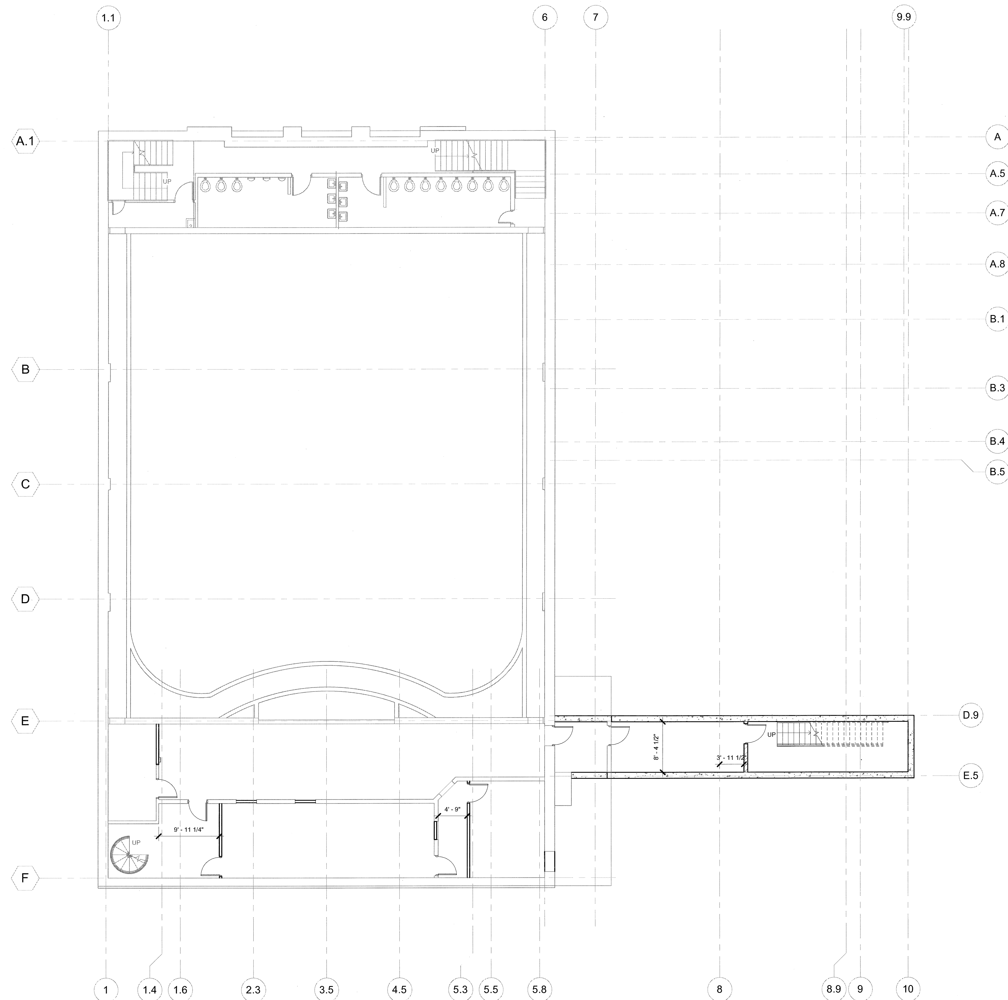
1 BASEMENT DIMENSION PLAN 1/8" = 1'-0"
