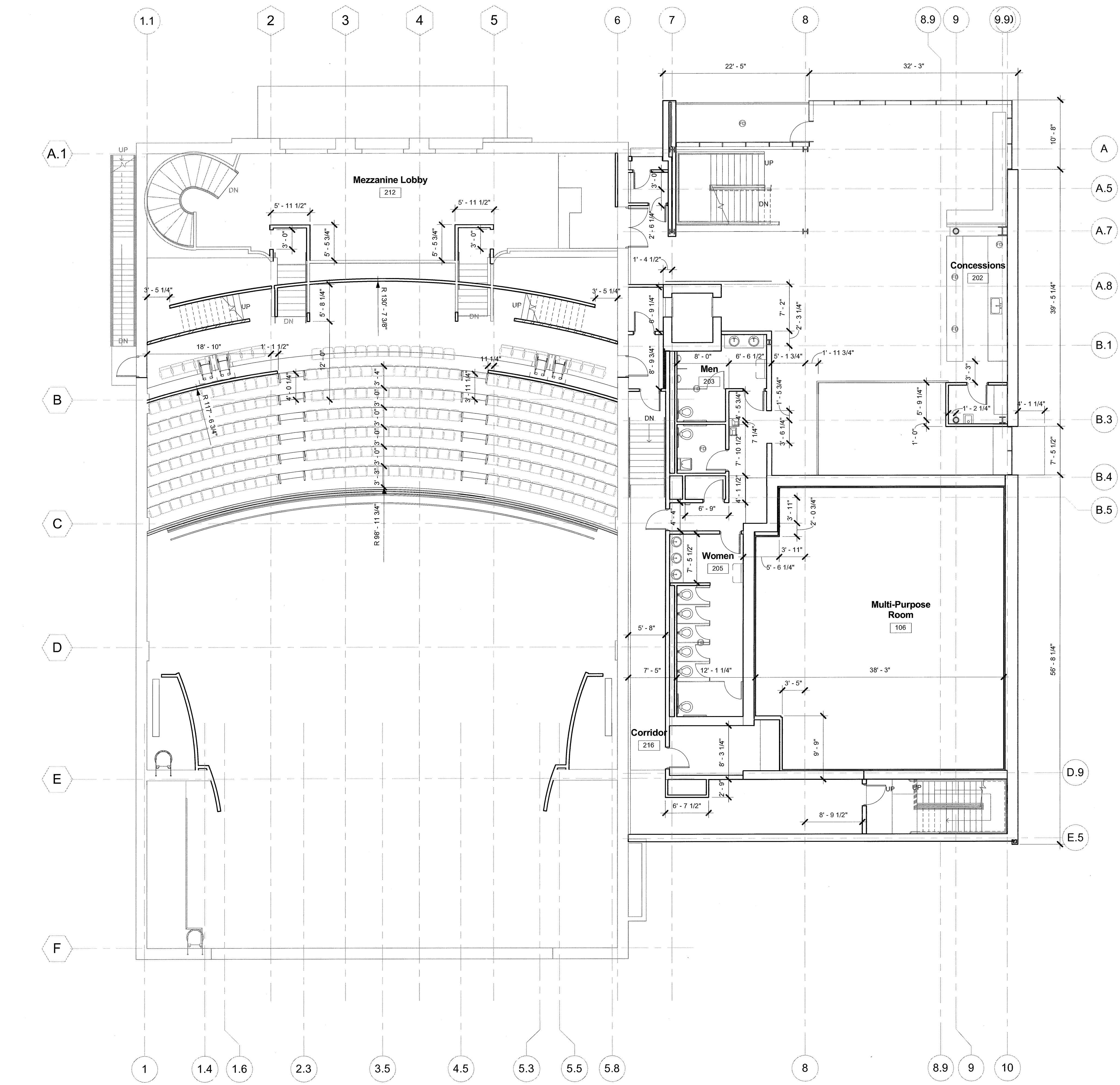
1 MEZZANINE DIMENSION PLAN 1/8" = 1'-0"
