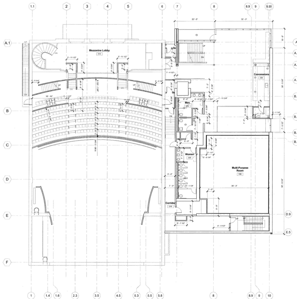
1 MEZZANINE DIMENSION PLAN
