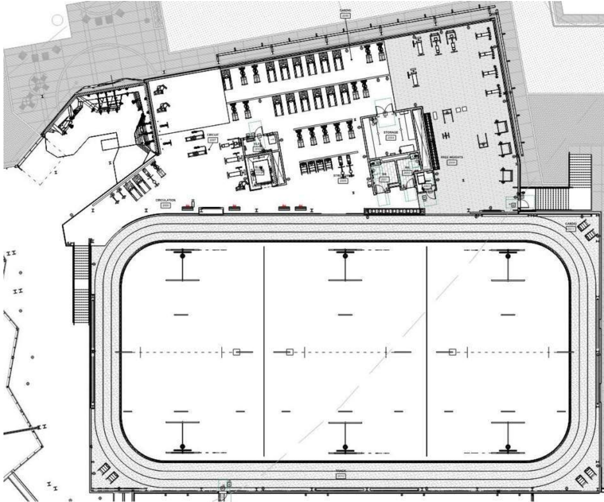
FURNITURE PLAN MEZZANINE AREA D
