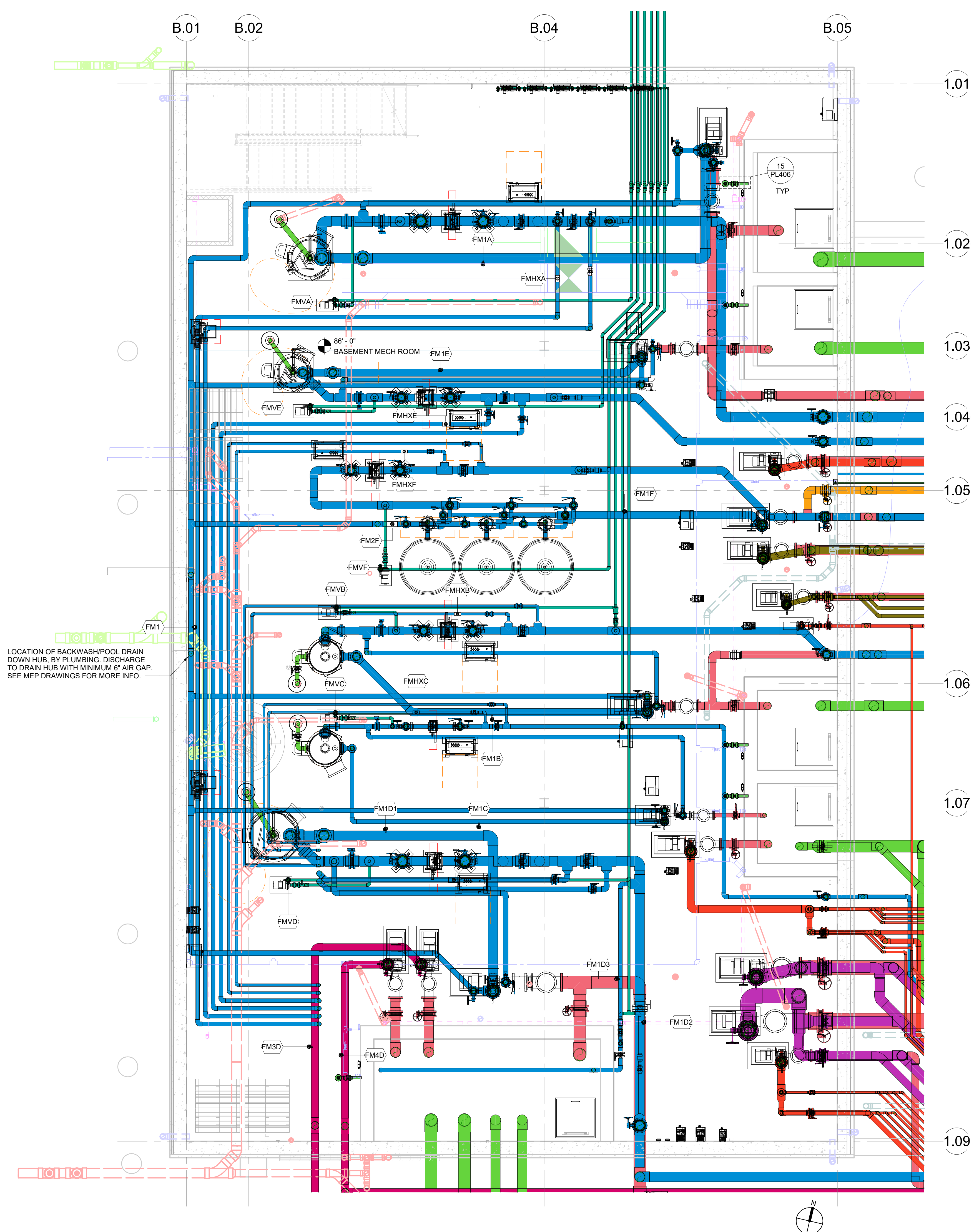
2 | BASEMENT MECHANICAL PIPING PLAN PLAN VIEW 1/4" = 1'-0"
