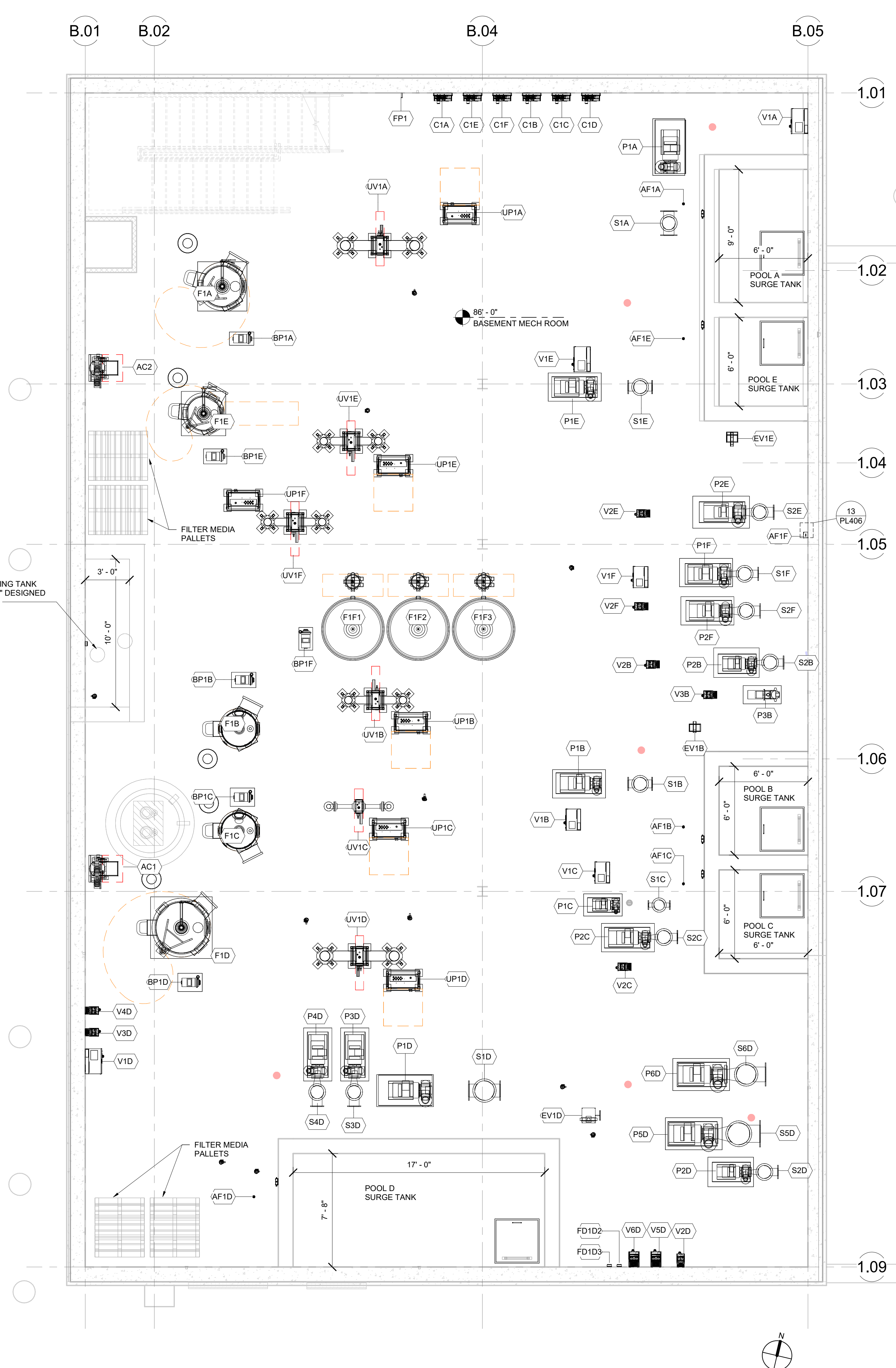
1 | BASEMENT MECHANICAL EQUIPMENT PLAN PLAN VIEW 1/4" = 1'-0"
