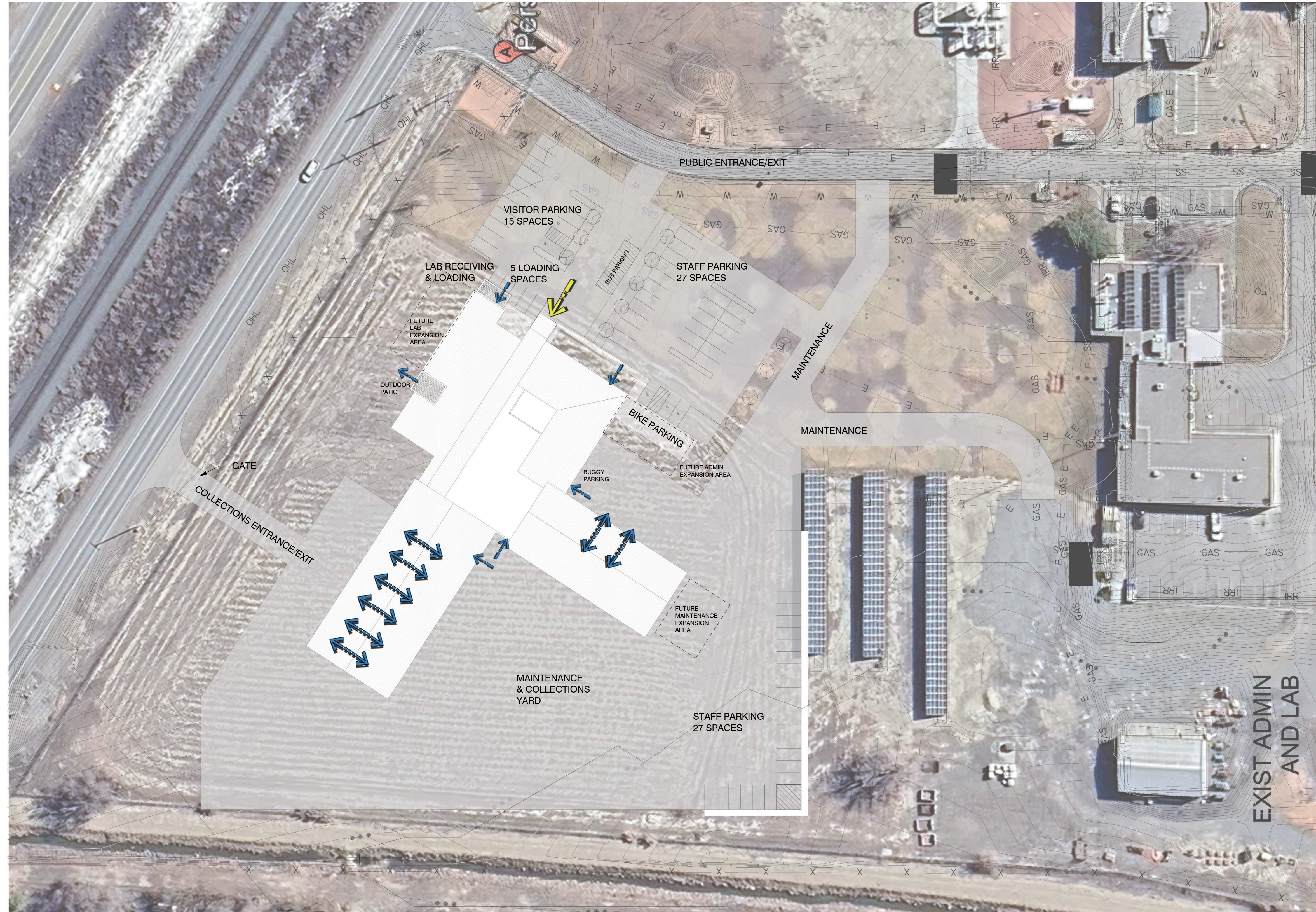
SD Site Plan 1" = 40'-0"
