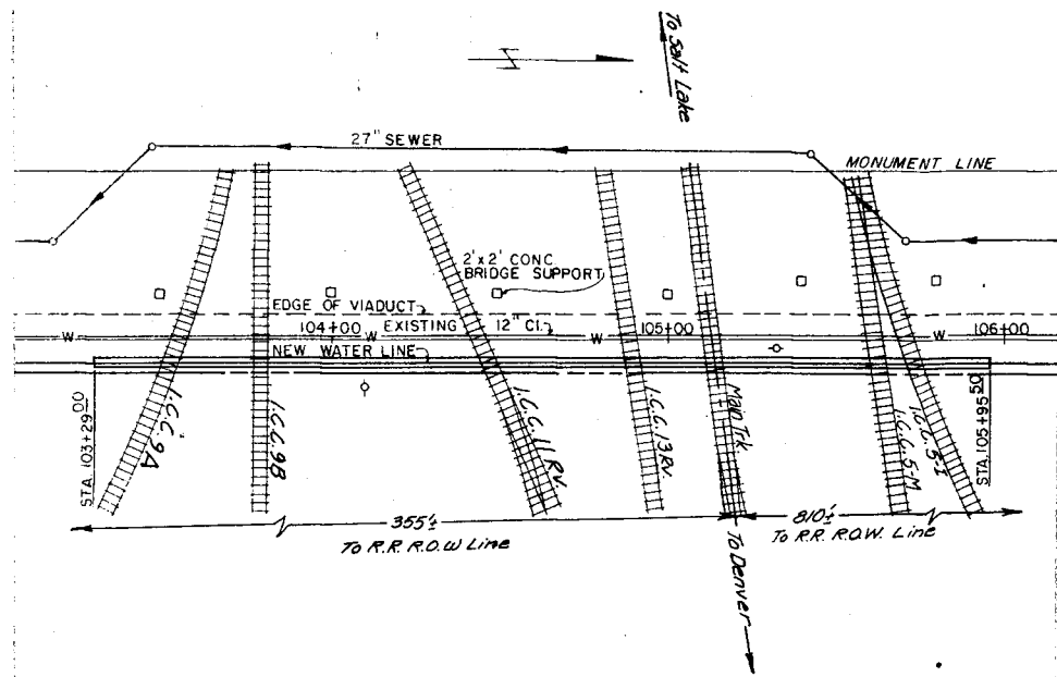
PLAN 1"=40'
