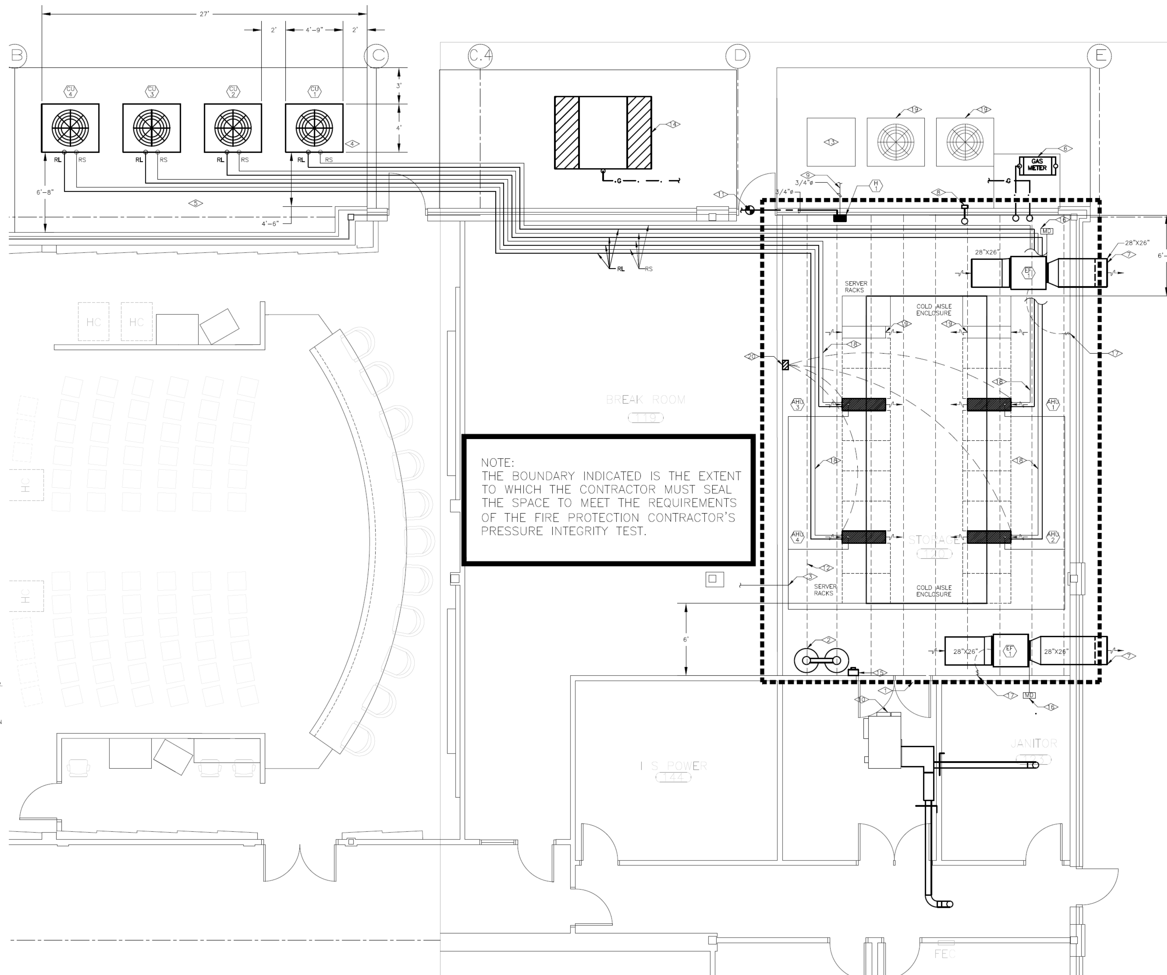
MECHANICAL FLOOR PLAN SCALE: 1/4"=1'-0" NORTH
