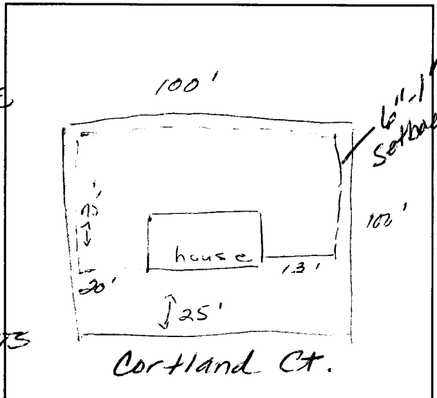
PLOT PLAN
