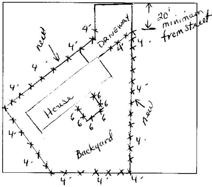
PLOT PLAN
