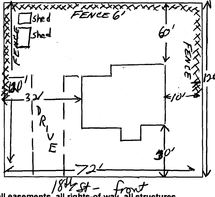
PLOT PLAN
