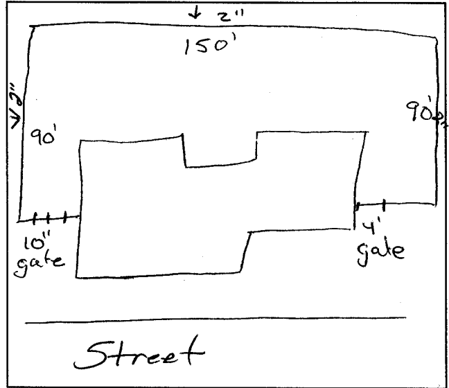
PLOT PLAN
