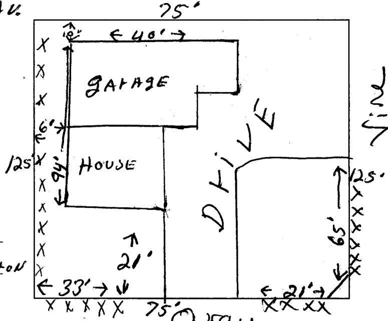
PLOT PLAN
