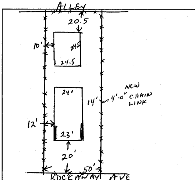
PLOT PLAN
