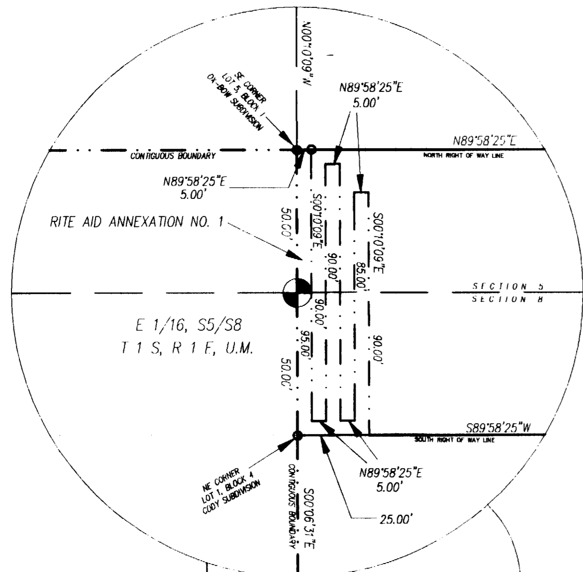
DETAIL NTS
