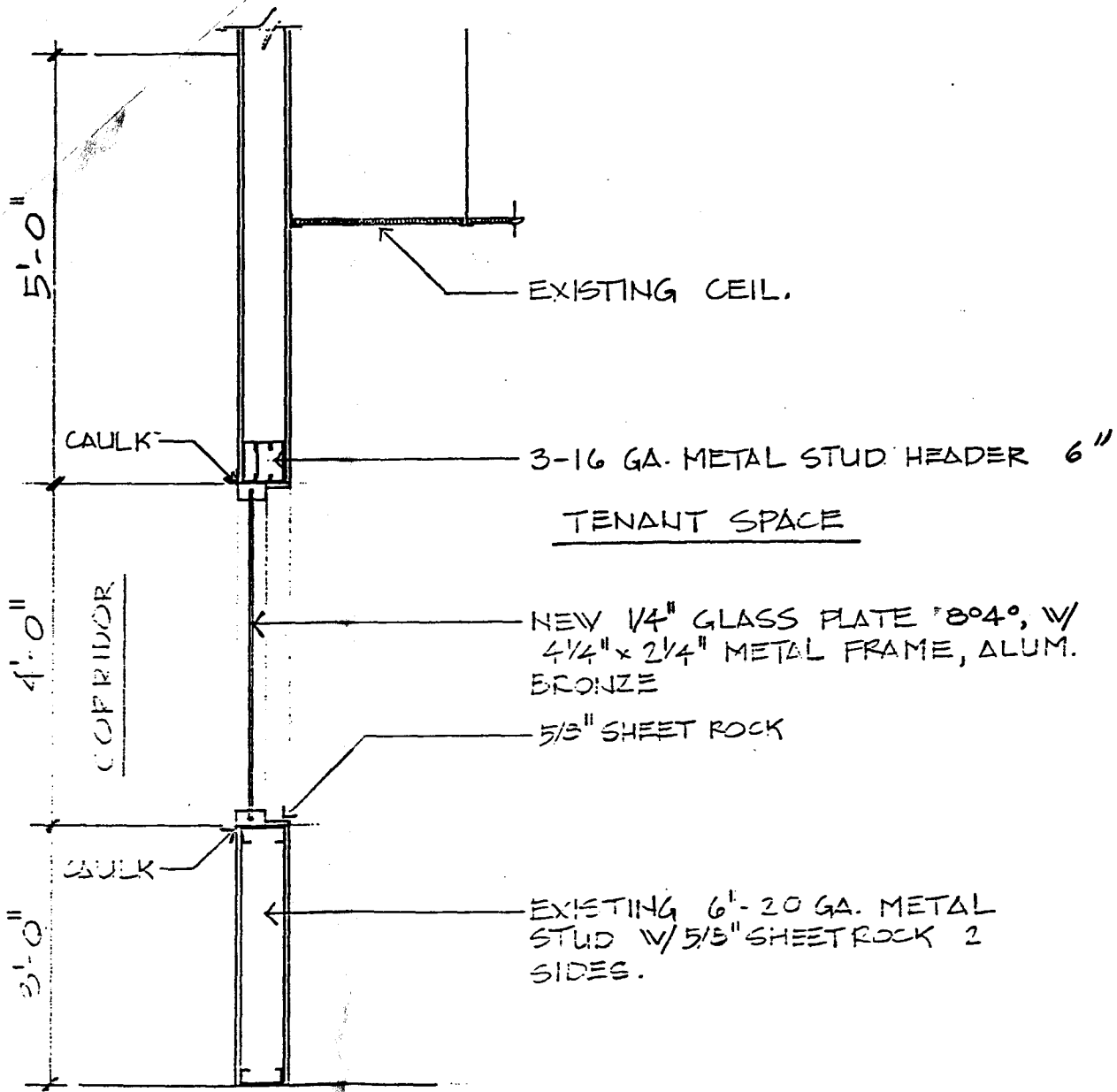
WALL SECTION \frac{1}{2}'' = 1'-0''
