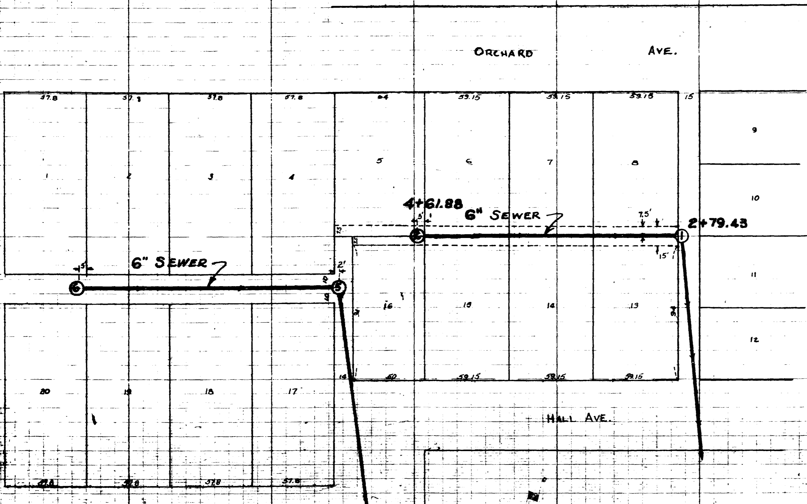
PLAN ALLEY BETWEEN HALL & ORCHARD AVENUES EAST HOLME-IN-GRANDVIEW SCALE 1"=40'
