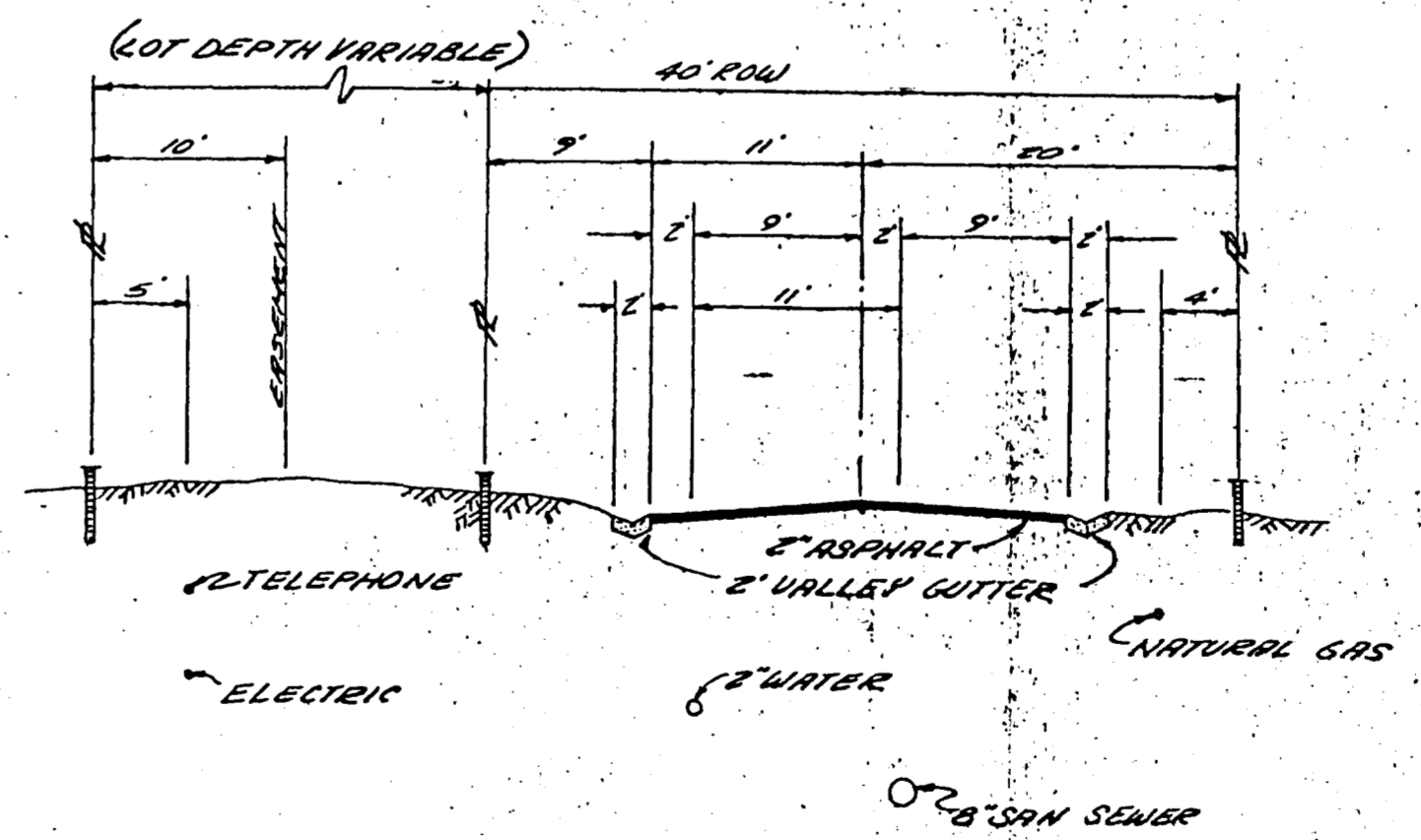
SECTION B-B 1"=10' HORIZ
