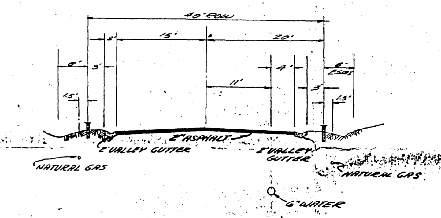
SECTION A-A 1"=10' HORIZ
