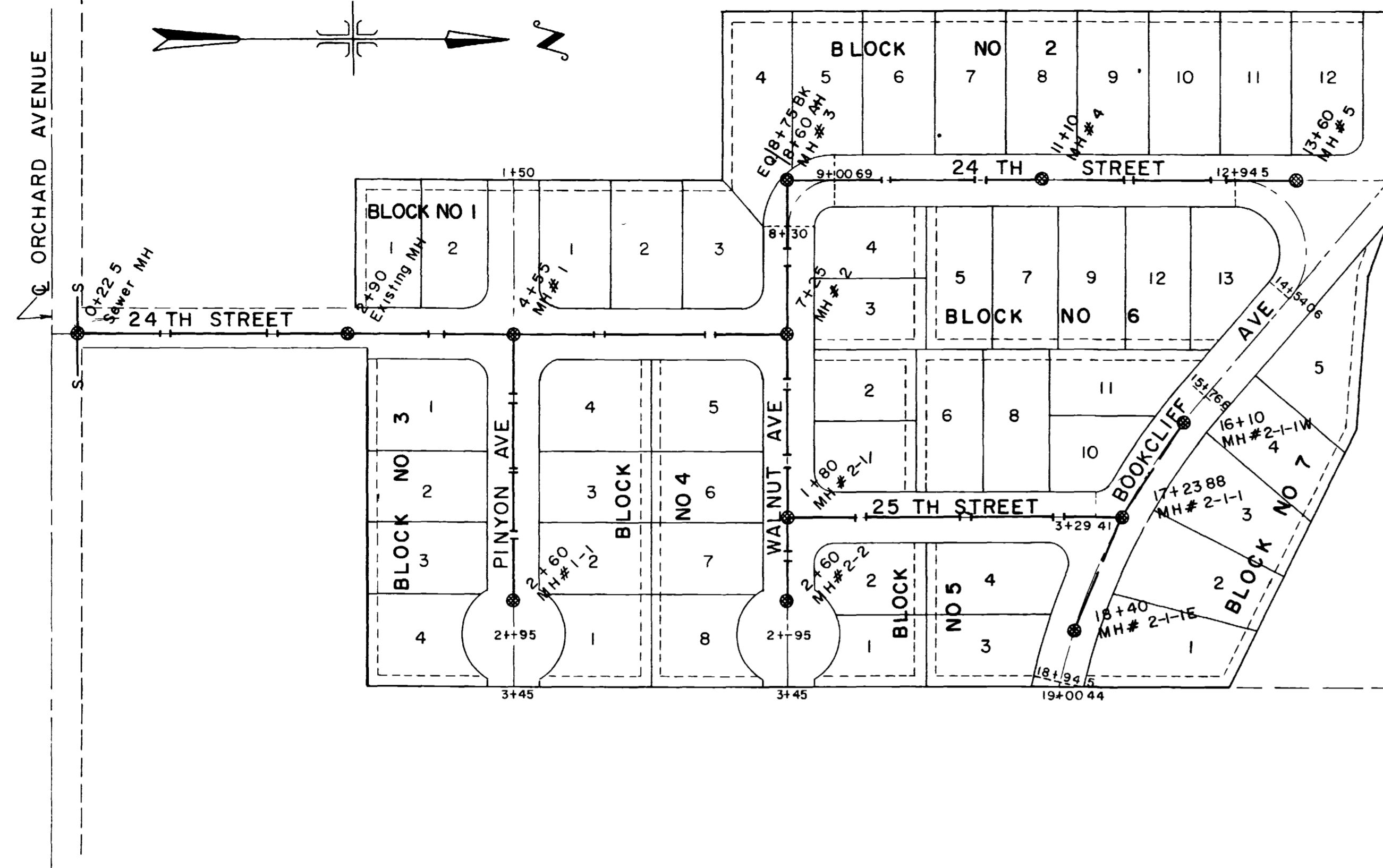
PLAN SCALE 1" = 100'
